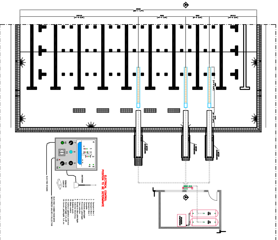
SWIMMING LANE POOL PLUMBING PLAN VIEW SCALE 1:50
